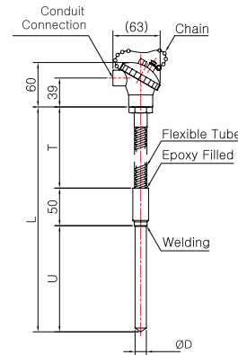
Model No. | SS-5049S (Sheath)
