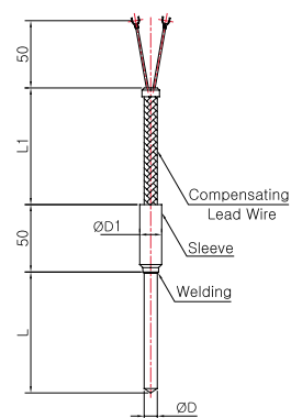
Model No. | SS-5048GD ( Sheath )
