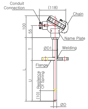
Model No. | SS-5046W-1-1 (Sheath Spring Load)
