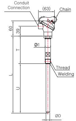
Model No. | SS-5044S-1-1 (Sheath Spring Load)
