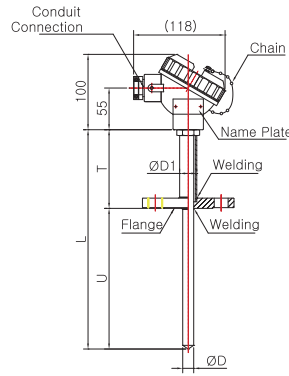
Model No. | SS-5046W-1 (Sheath)
