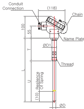
Model No. | SS-5044W-1-1 (Sheath Spring Load)
