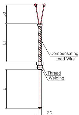
Model No. | SS-5048GD-1 ( Compensating Lead Wire )
