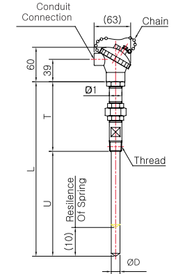
Model No. | SS-5044S-2-1 (Sheath Spring Load)
