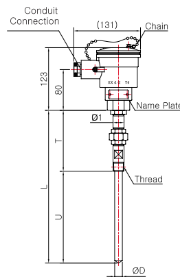
Model No. | SS-5044E-2 (Sheath)
