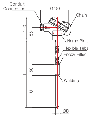
Model No. | SS-5049W (Sheath)
