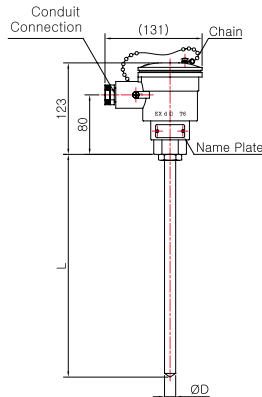
Model No. | SS-5041E (Sheath)
