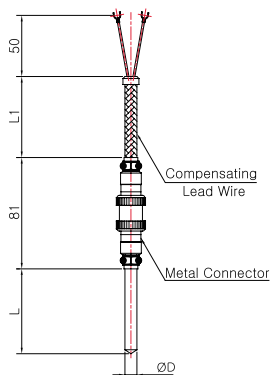
Model No. | SS-5048GH ( Metal Connector )
