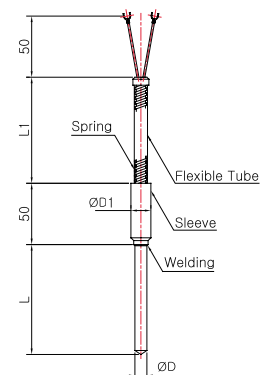
Model No. | SS-5048GE ( Flexible Tube )
