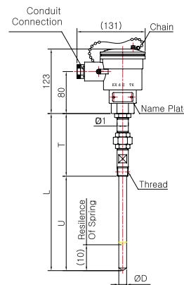
Model No. | SS-5044E-2-1 (Sheath Spring Load)
